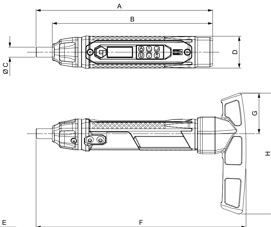
ProTronic® Plus 9 comes supplied with L shaped handle for easier torque application
