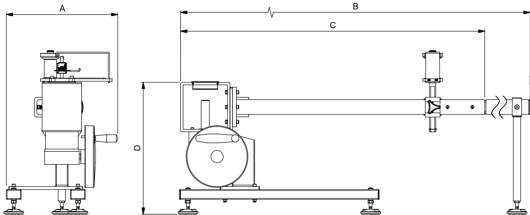
20506 ISO 3,000 N-m Motorised Loader
